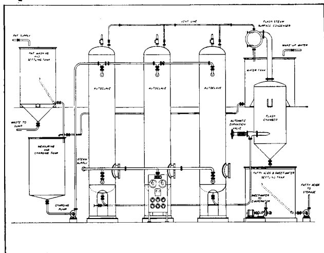
WURSTER & SANGER AUTOCLAVE FAT SPLITTING PLANT
